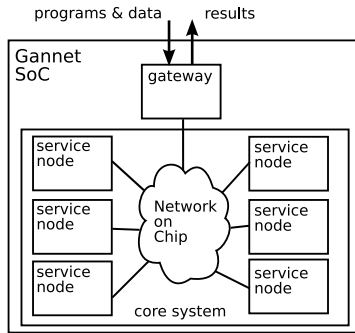
Figure 1. Gannet architecture
